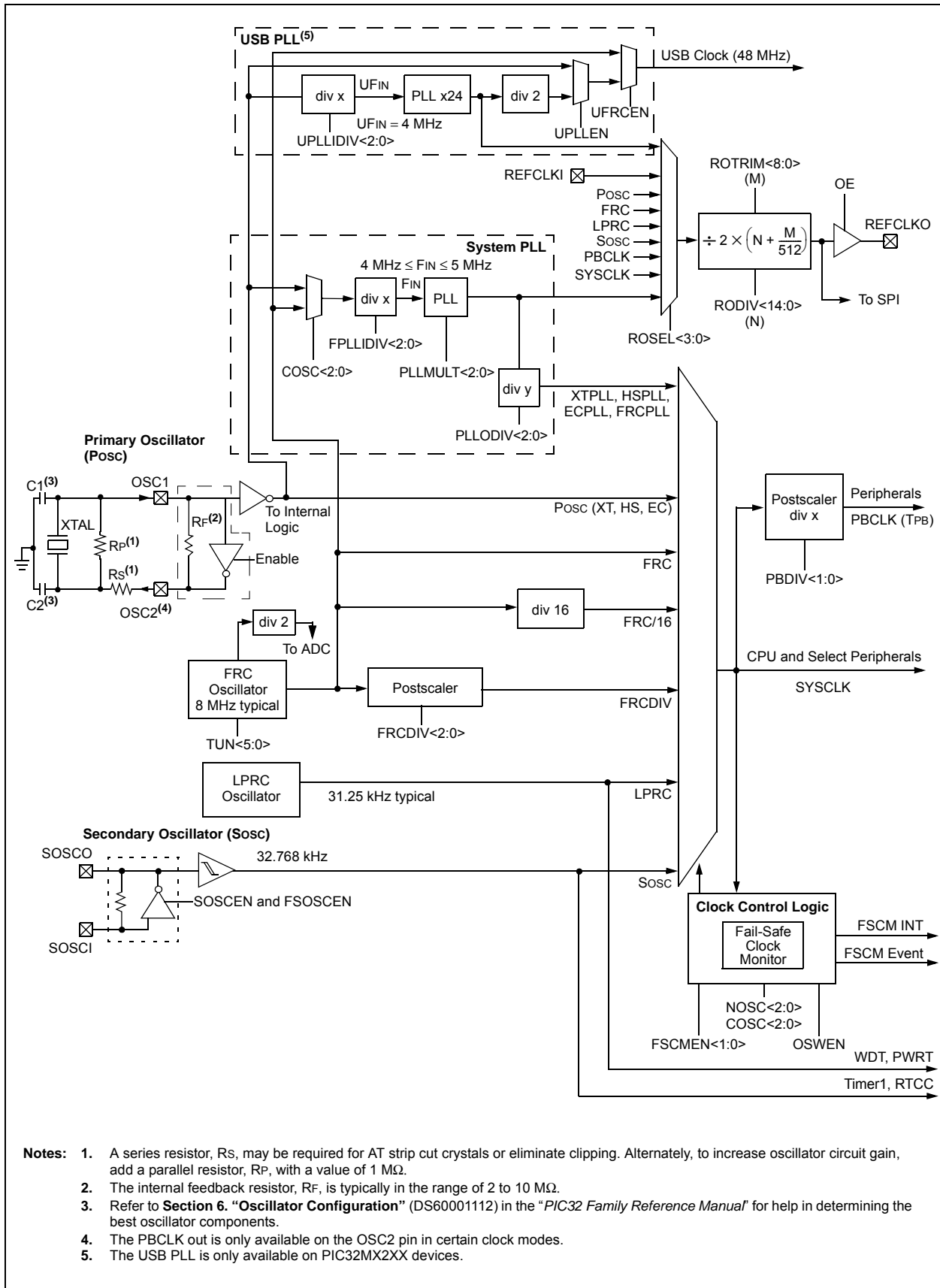
FIGURE 8-1: OSCILLATOR DIAGRAM
